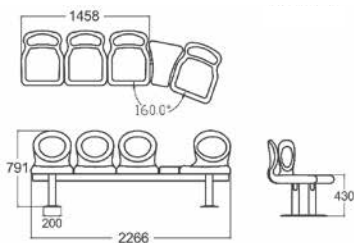
V04-1420 VIA LUXOR QUADRUPLE SERIES (4 POSITIONS R/H CURVE)
